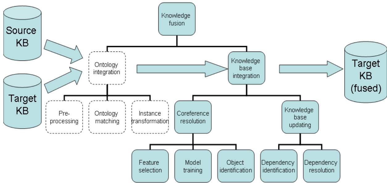
Fig.3.1 Illustration of the Semantics Based Level Wise Knowledge Base Database Integration Architecture
